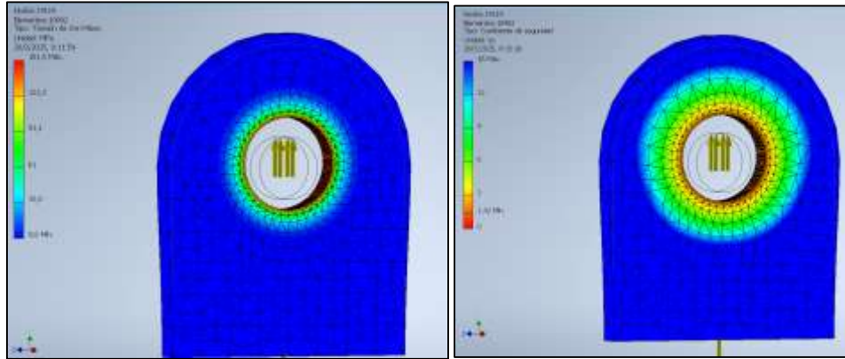
Figure 10. Von Mises Stress and Safety Factor
