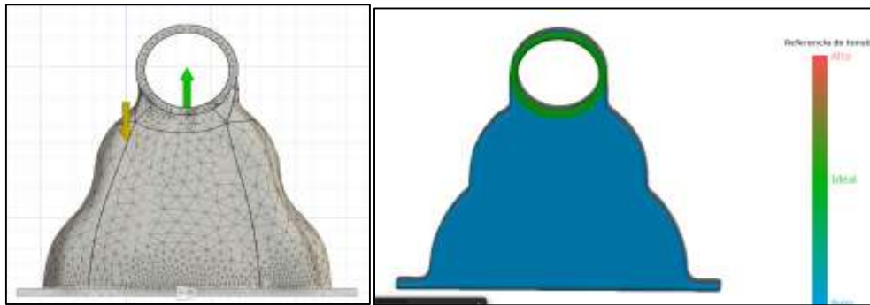
Figure 12. Von Mises Stress Result for 3-Axis Milling
