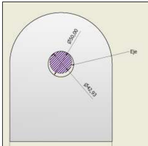
Figure 2. Distributed Load on the Lifting Lug
