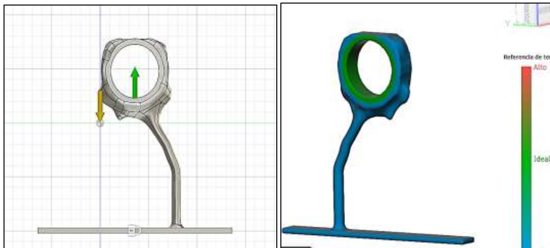
Figure 11. Von Mises Stress Result for Additive Manufacturing
