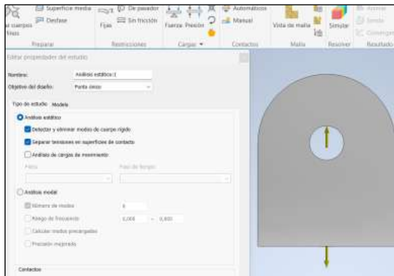
Figure 3. Definition of Loads and Constraints
