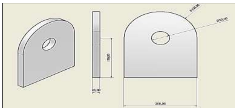
Figure 1. Lifting Lug Dimensions Measured in (mm).
