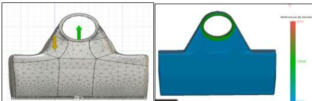
Figure 13. Von Mises Stress Result for Casting
