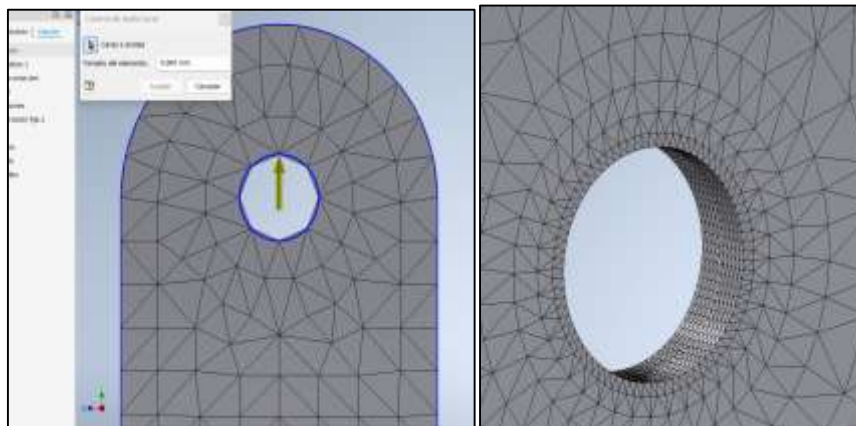
Figure 4. Mesh Configuration by Zones
