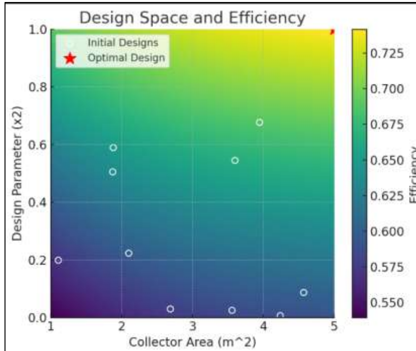
Figure 3. Collector design space (area vs. enhancement level) with simulated efficiency map. White circles represent the initially evaluated (random) designs, while the red star indicates the optimal design discovered by the generative model. The background colors show thermal efficiency (right-hand color bar) according to the combination of area and geometric enhancements: higher efficiencies are observed in the corner with large area and high enhancement level (yellow), matching the location of the identified optimal design.
